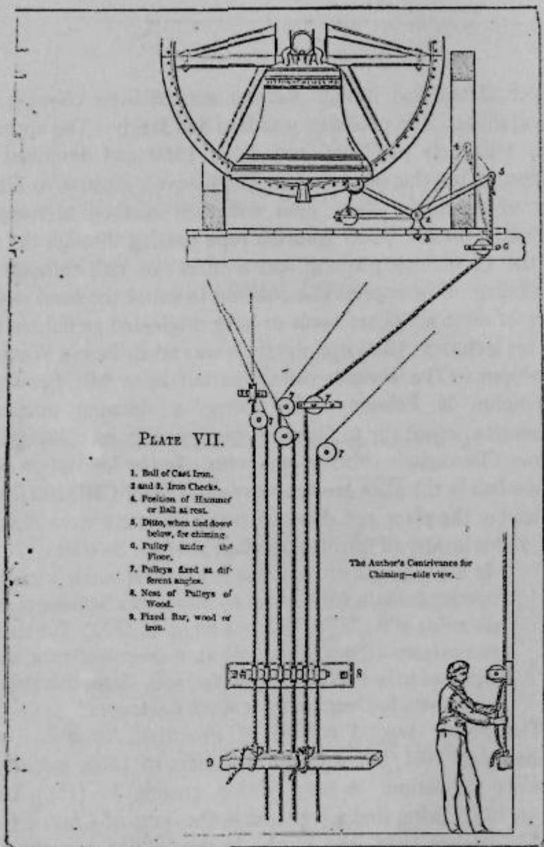
The plate made from Ellacombe's drawing of his hammers, afterwards plagiarised by Warners.
